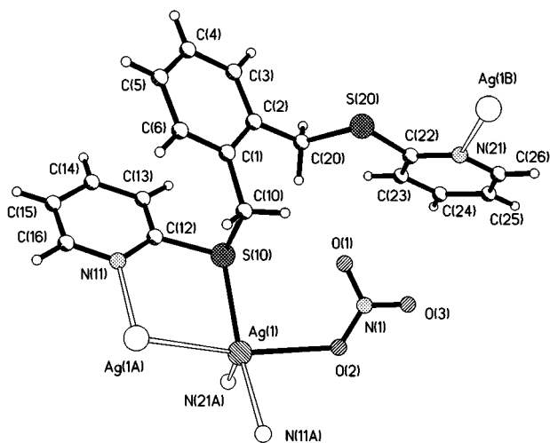
Fig. 5 Perspective view and atom labelling of complex 4 . Selected interatomic distances (Å) and angles ( ^{\circ} ): Ag(1)–Ag(1A) 2.9874(5), Ag(1)–N(11A) 2.288(2), Ag(1)–N(21A) 2.377(2), Ag(1)–S(10) 2.4984(8), Ag(1)–O(2) 2.571(2); Ag(1A)–Ag(1)–N(11A) 90.79(6), Ag(1A)–Ag(1)–N(21A) 117.51(6), Ag(1A)–Ag(1)–S(10) 78.35(2), Ag(1A)–Ag(1)–O(2) 155.46(6), N(11A)–Ag(1)–N(21A) 103.82(8), N(11A)–Ag(1)–S(10) 154.44(6), N(11A)–Ag(1)–O(2) 85.09(8), N(21A)–Ag(1)–S(10) 101.71(6), N(21A)–Ag(1)–O(2) 86.91(8), S(10)–Ag(1)–O(2) 95.21(5).
